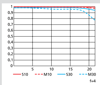
Schéma MTF (Modulation Transfer Function)
